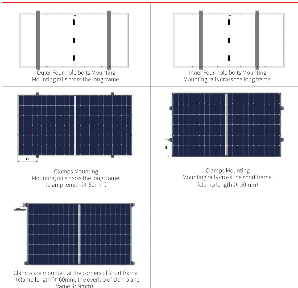
Figure 6 Monofacial Module Installation Annex
